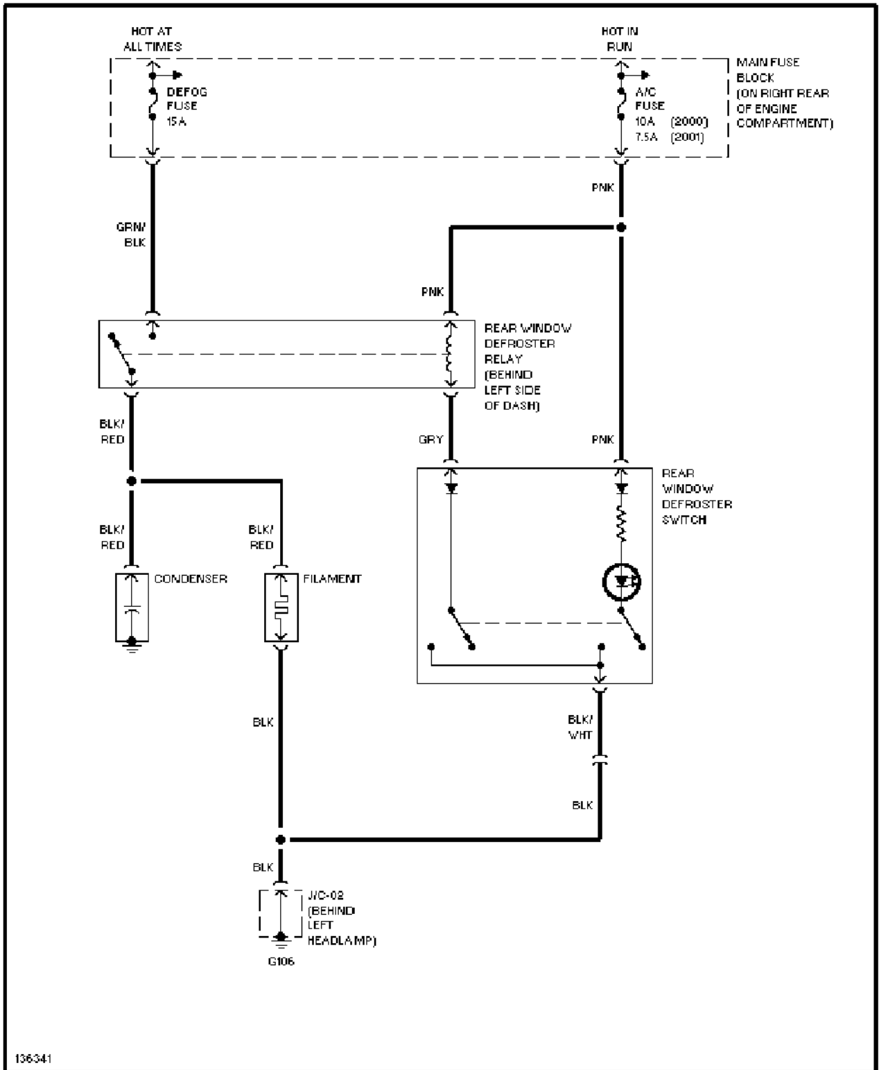
Defogger Circuit
