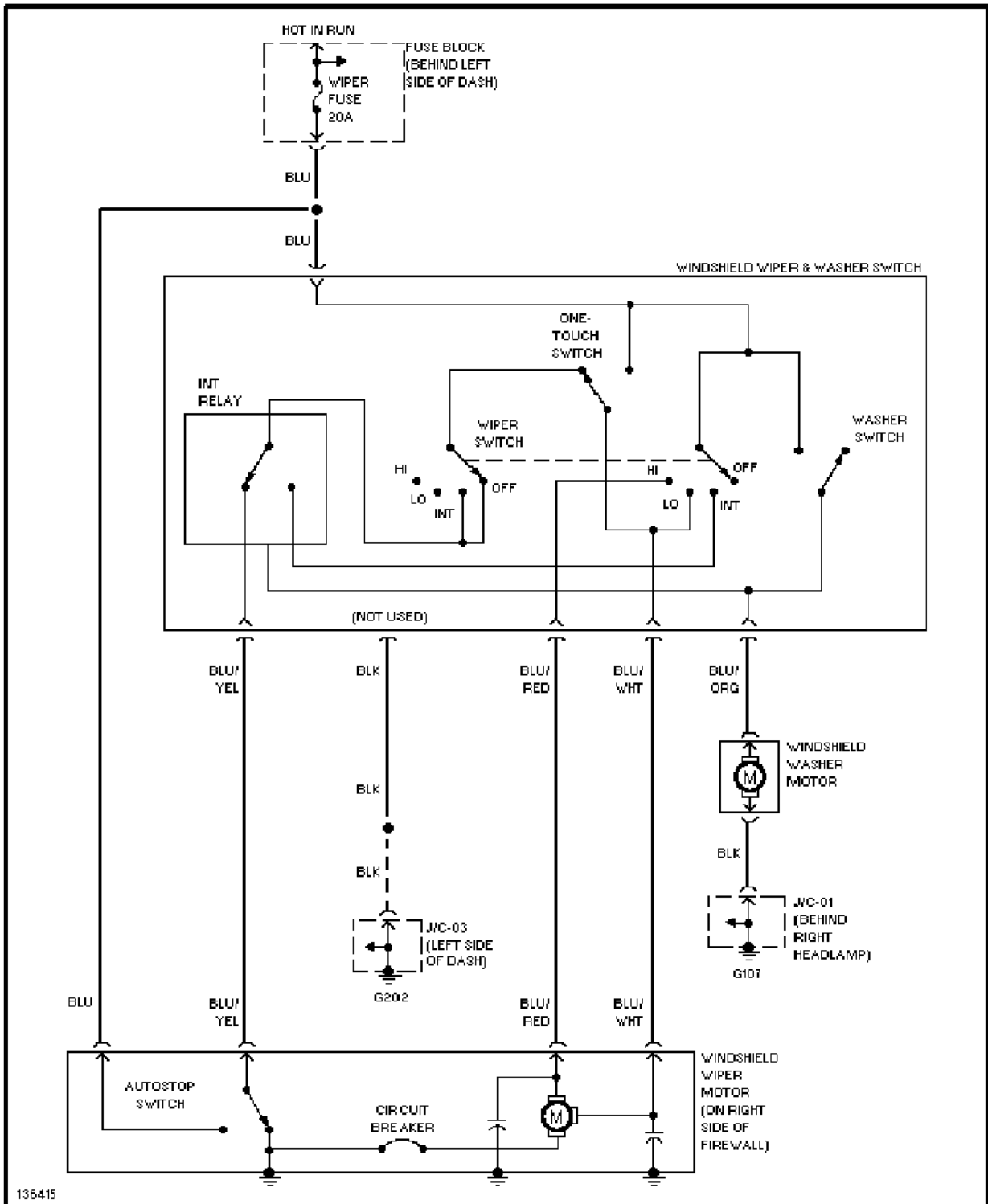
Wiper/Washer Circuit
