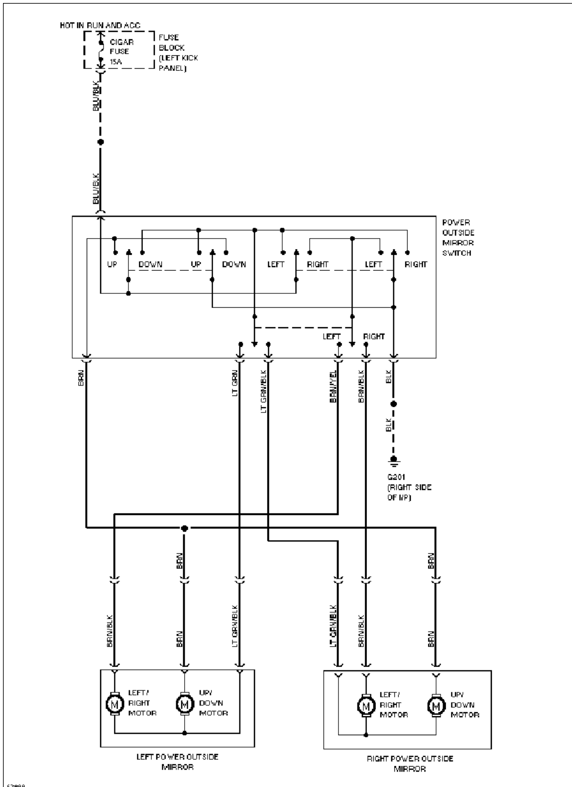
Power Mirror Circuit
