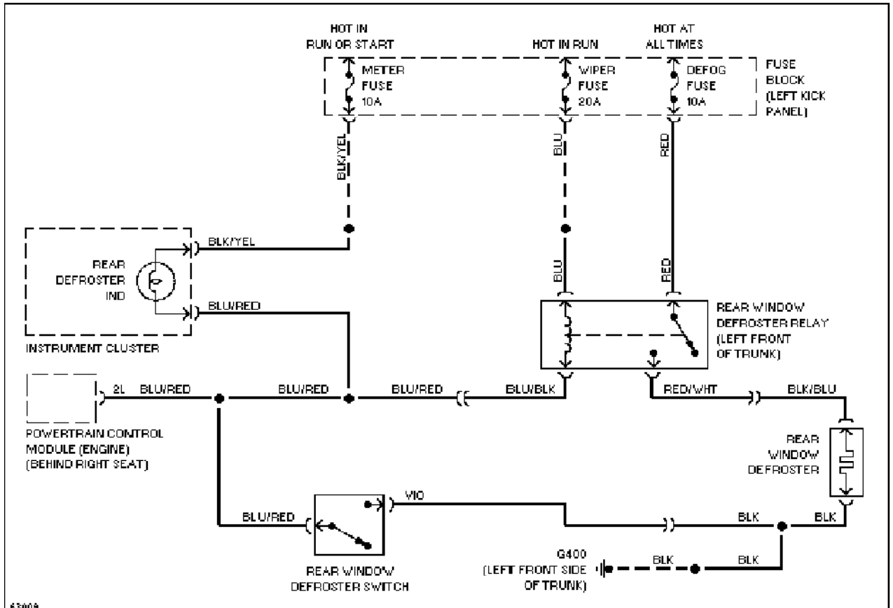
63009 Defogger Circuit
