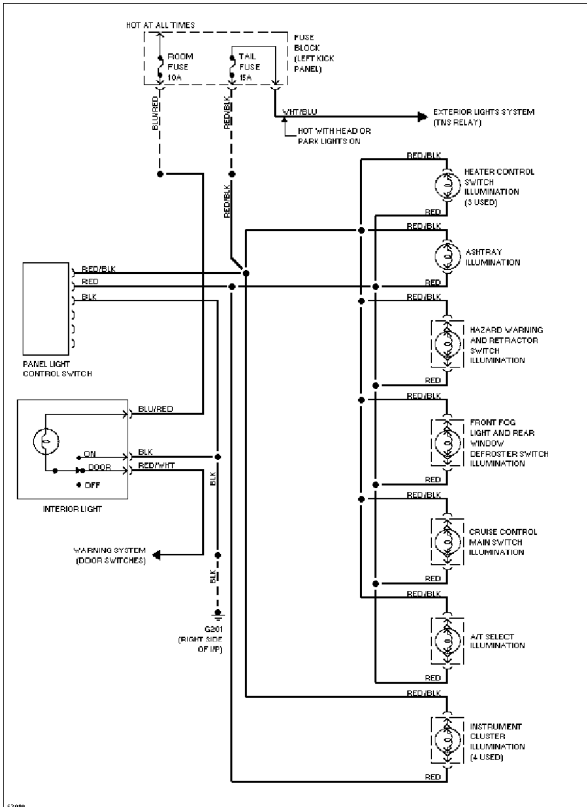
Interior Light Circuit
