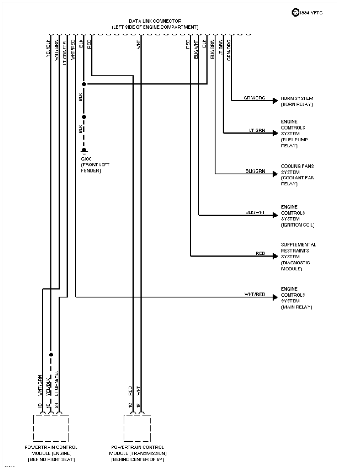
Data Link Connector Circuit
