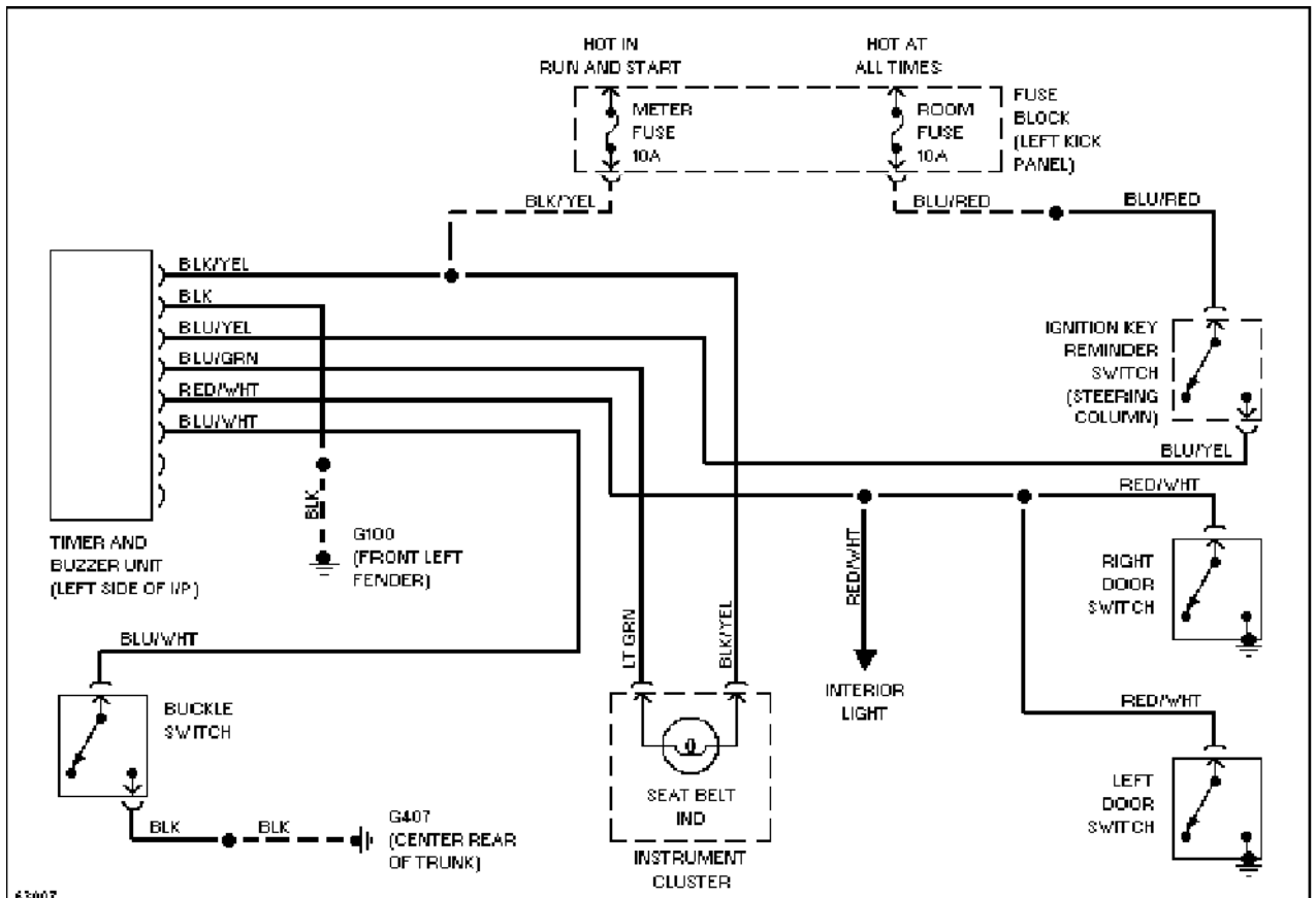
Warning System Circuits
