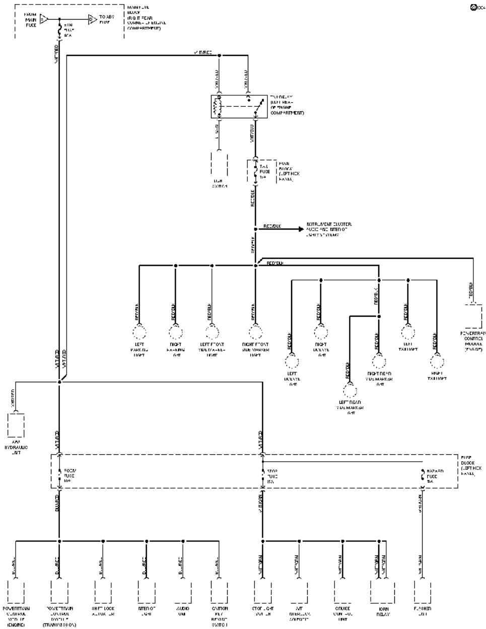
Power Distribution Circuit (2 of 3)
