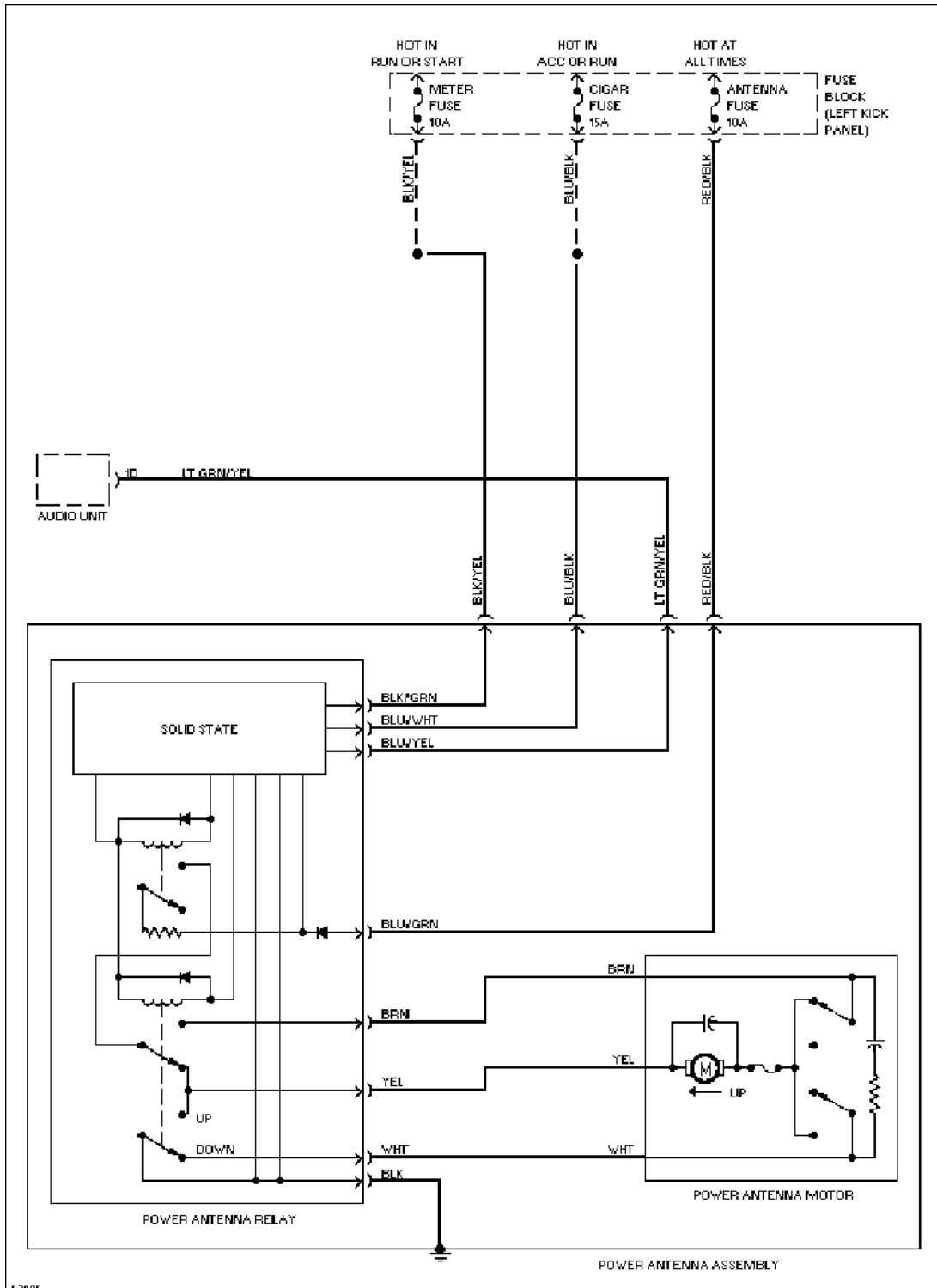
Power Antenna Circuit
