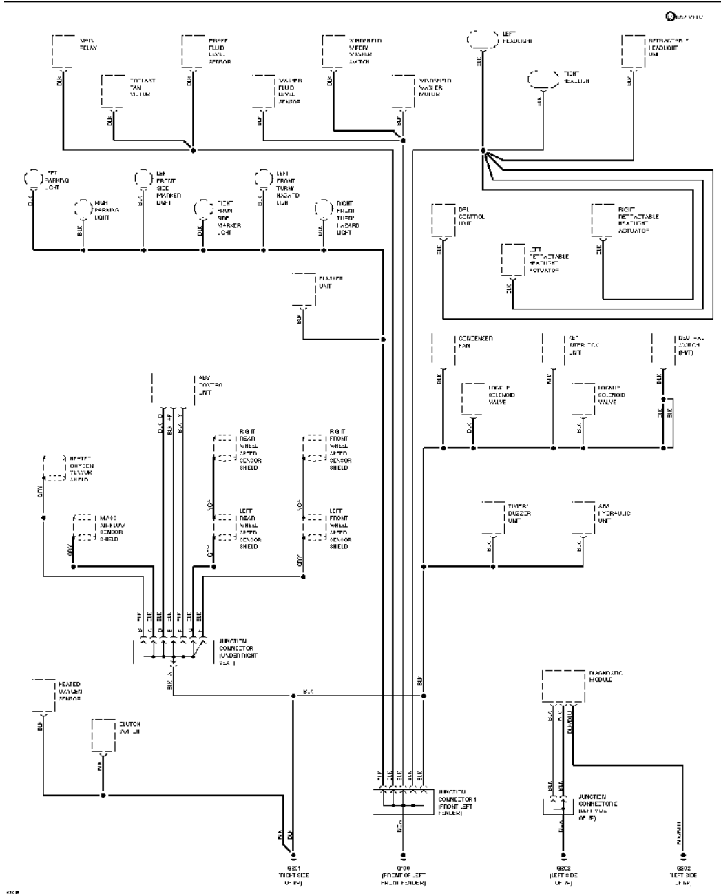
Ground Distribution Circuit (1 of 2)
