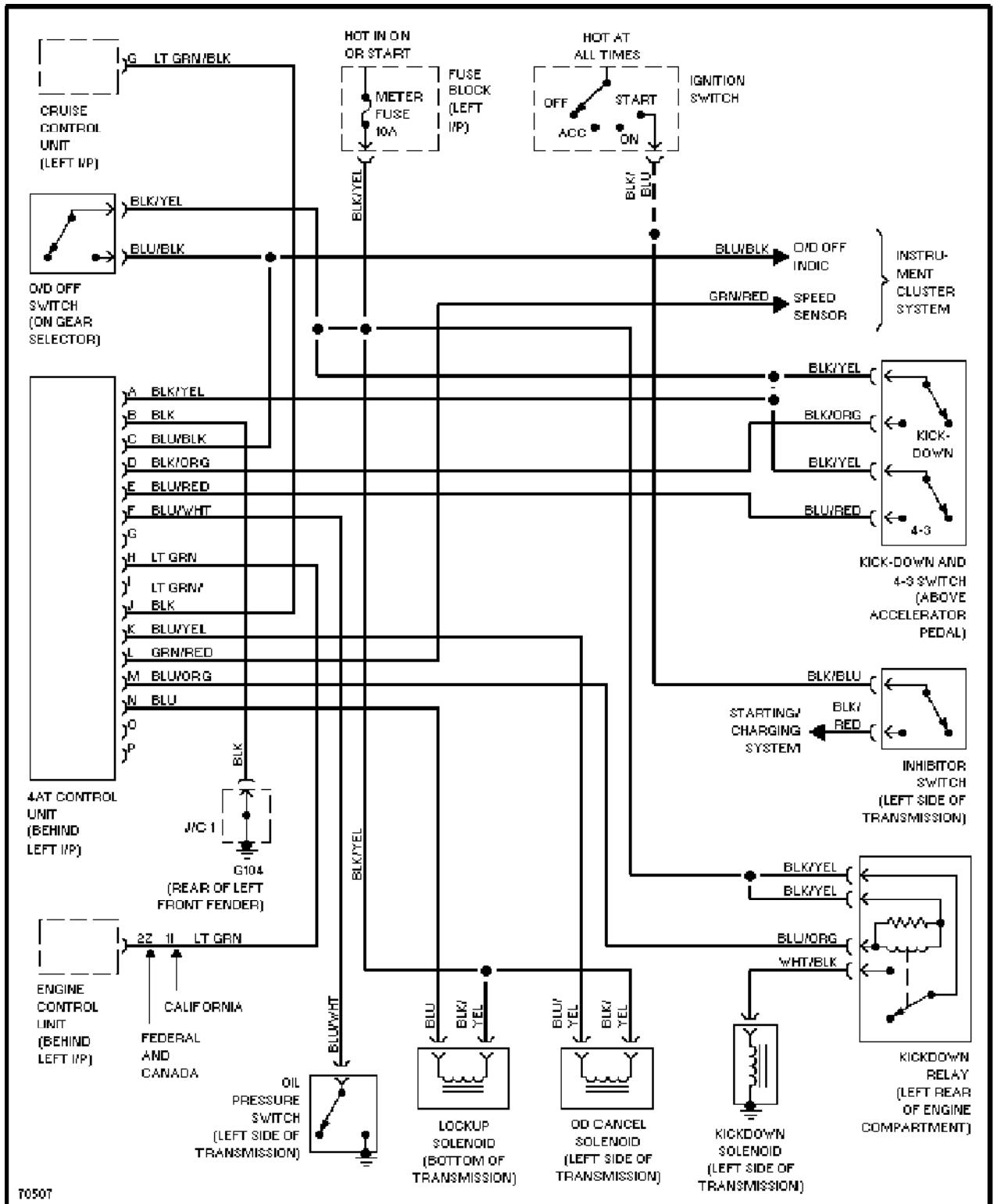
Transmission Circuit
