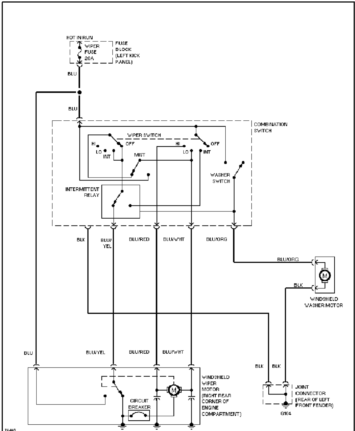
Wiper/Washer Circuit
