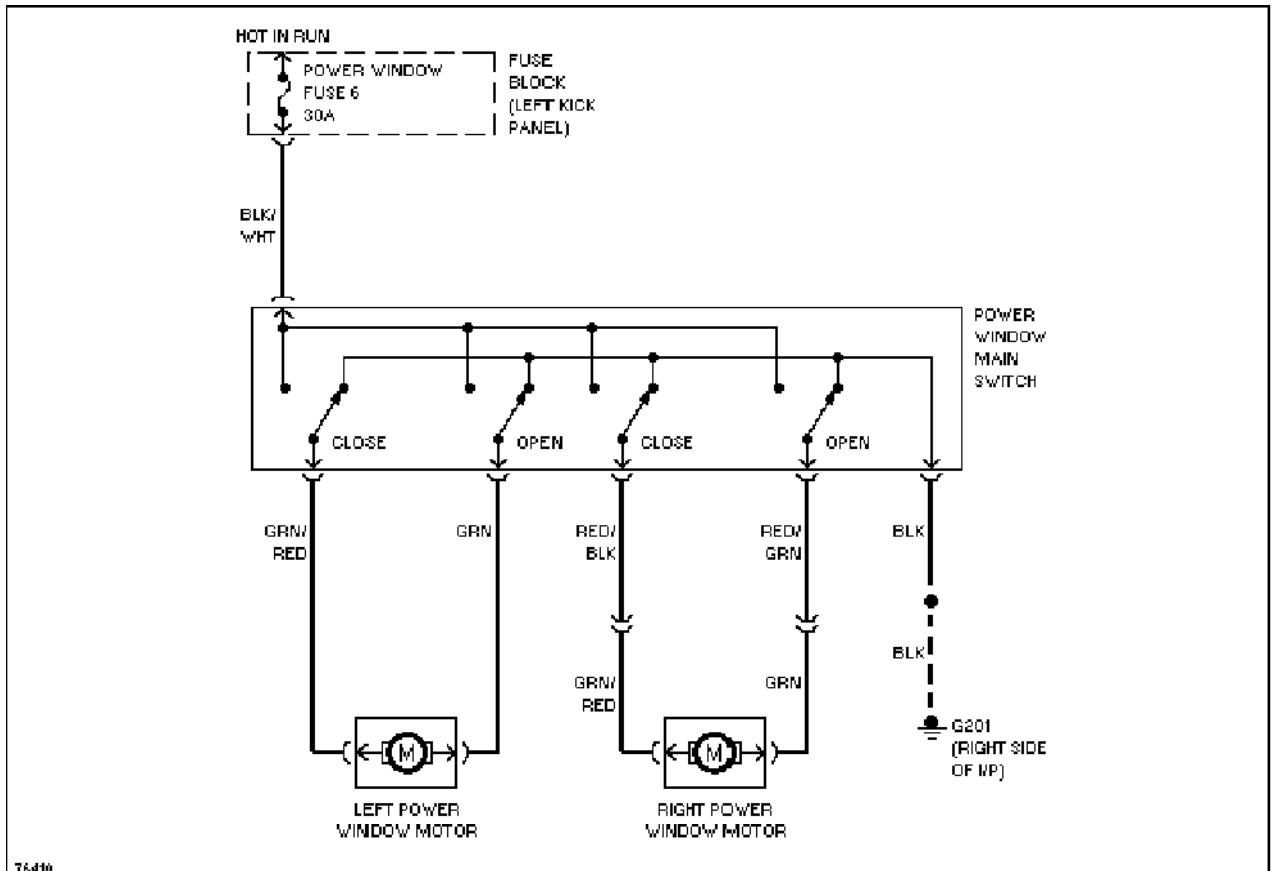
Power Window Circuit
